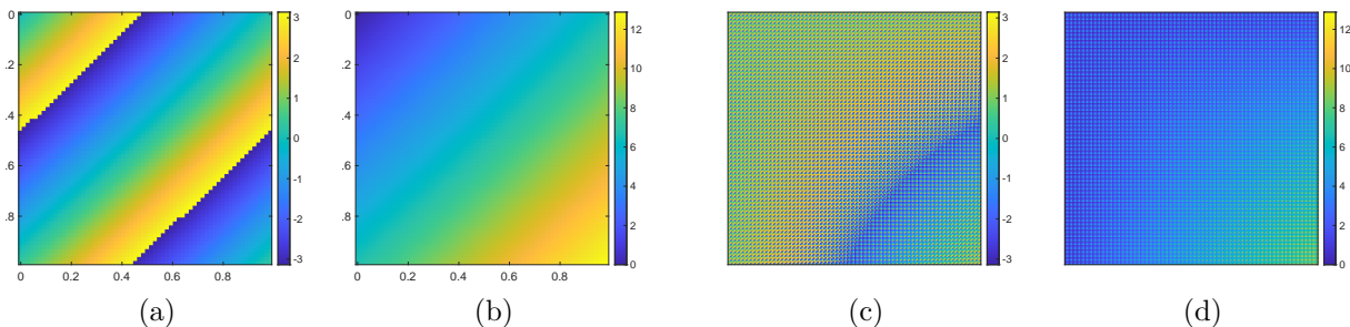
Figure 11: Phase recovery results for the 2D uniform FIO given in (34). N = 64^2 is the size of the phase matrix (\Phi(x, \xi))_{x \in X, \xi \in \Omega} . (a) A row vector of the phase matrix before recovery and reshaped into a matrix of size 64 \times 64 . (b) A recovered row vector of the phase matrix when it is reshaped into a matrix of size 64 \times 64 . (c) The phase matrix of size 64^2 \times 64^2 before recovery. (d) The recovered phase matrix of size 64^2 \times 64^2 .
