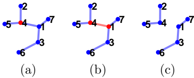
Figure 4: (a) An MST \mathcal{T}(\mathcal{X}) with a discontinuity location at Node 4. (b) Separate \mathcal{T}(\mathcal{X}) at the edge between Node 4 and its predecessor Node 1. (c) Two resulting subtrees and the corresponding recovery path matrices [1, 3; 1, 7; 3, 6] and [4, 2; 4, 5] .
