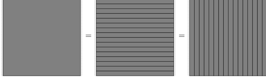
Figure 8: The left figure is a complementary two-dimensional low-rank kernel matrix K . Assume that the depth of the quadtrees of column and row spaces is 3. The middle figure illustrates the root-leaf partitioning that divides the row index set into 16 subsets as 16 leaves. The right one is for the leaf-root partitioning that divides the column index set into 16 subsets as 16 leaves.
