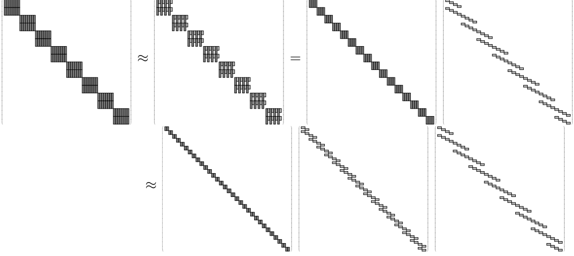
Figure 4: The recursive factorization of U^3 in Figure 3. Gray factors are matrices inheriting the low-rank property of the butterfly matrix. Top: left matrix: U^3 with each diagonal block partitioned into smaller blocks according to Equation (13) as indicated by black rectangles; middle-left matrix: low-rank approximations of submatrices in U^3 given by Equation (15); middle right matrix: U^4 ; right matrix: G^3 . Bottom: U^4 in the first row is further factorized into U^4 \approx U^5 G^4 , giving U^3 \approx U^5 G^4 G^3 .
